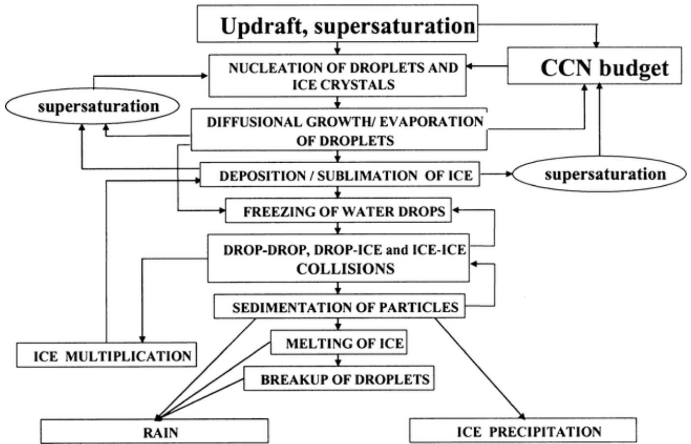
FIG. 1. Scheme of microphysical processes used in spectral (bin) microphysics model.
